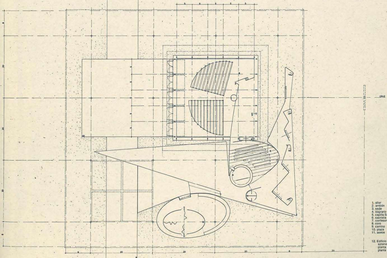
planta principal/main floor plan
